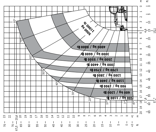
Rotation on lowered stabilizers with 1500 kg jib
