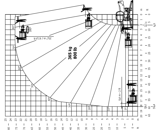
Rotation on lowered stabilizers with 365 kg platform
